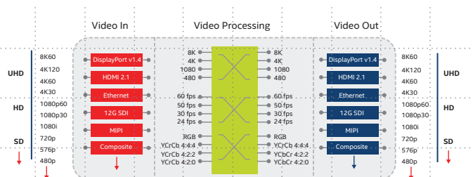
Figure 2. Intel® FPGA pre-canned video processing blocks are system verified to convert any incoming resolution and frame rate to any output
